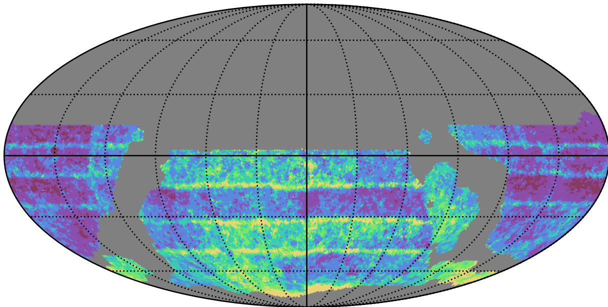
weather_cloudso6v3.4_10yrs WFD r band: Median Inter-Night Gap
