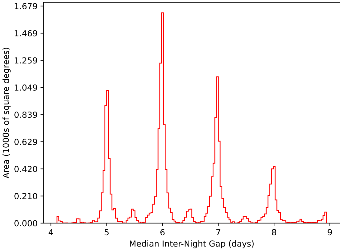
weather_cloudso6v3.4_10yrs WFD i band: Median Inter-Night Gap
