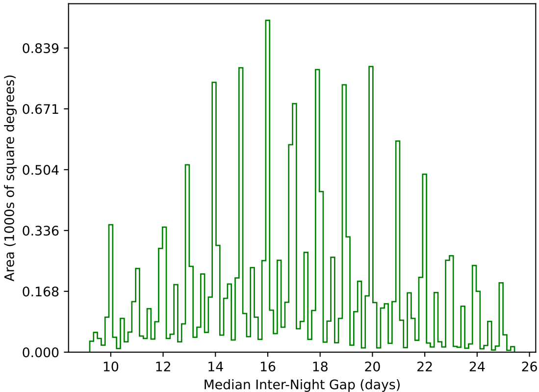
weather_cloudso6v3.4_10yrs WFD g band: Median Inter-Night Gap
