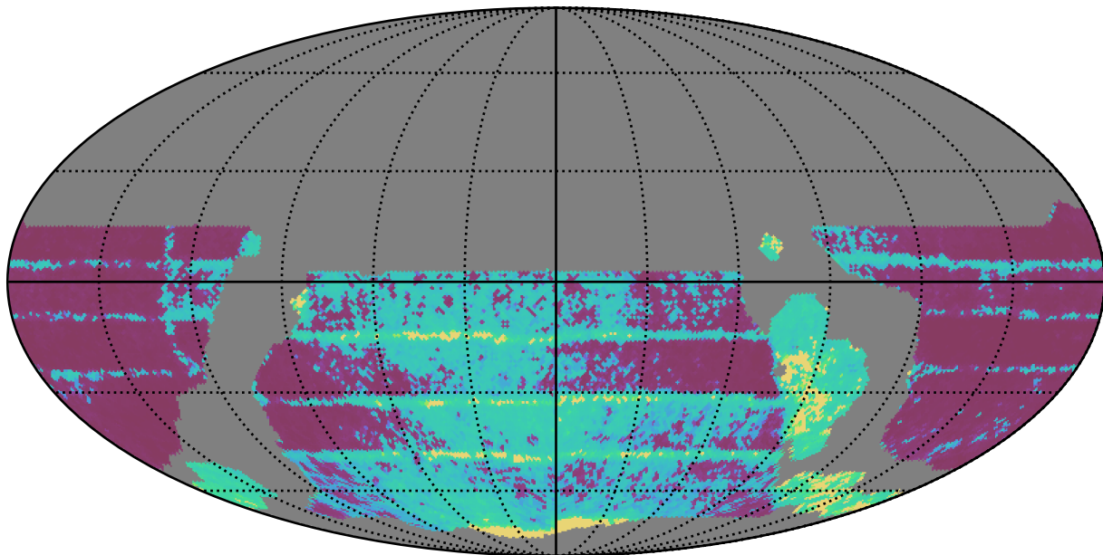
weather_cloudso6v3.4_10yrs WFD all bands: Median Inter-Night Gap
