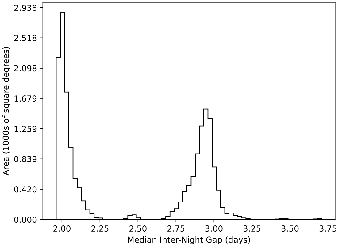
weather_cloudso6v3.4_10yrs WFD all bands: Median Inter-Night Gap
