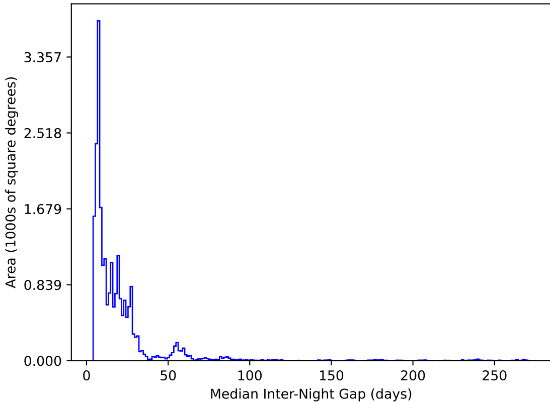
weather_cloudso6v3.4_10yrs All sky y band: Median Inter-Night Gap
