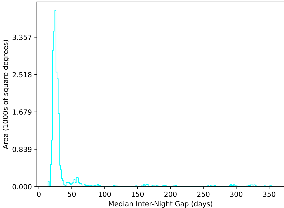
weather_cloudso6v3.4_10yrs All sky u band: Median Inter-Night Gap
