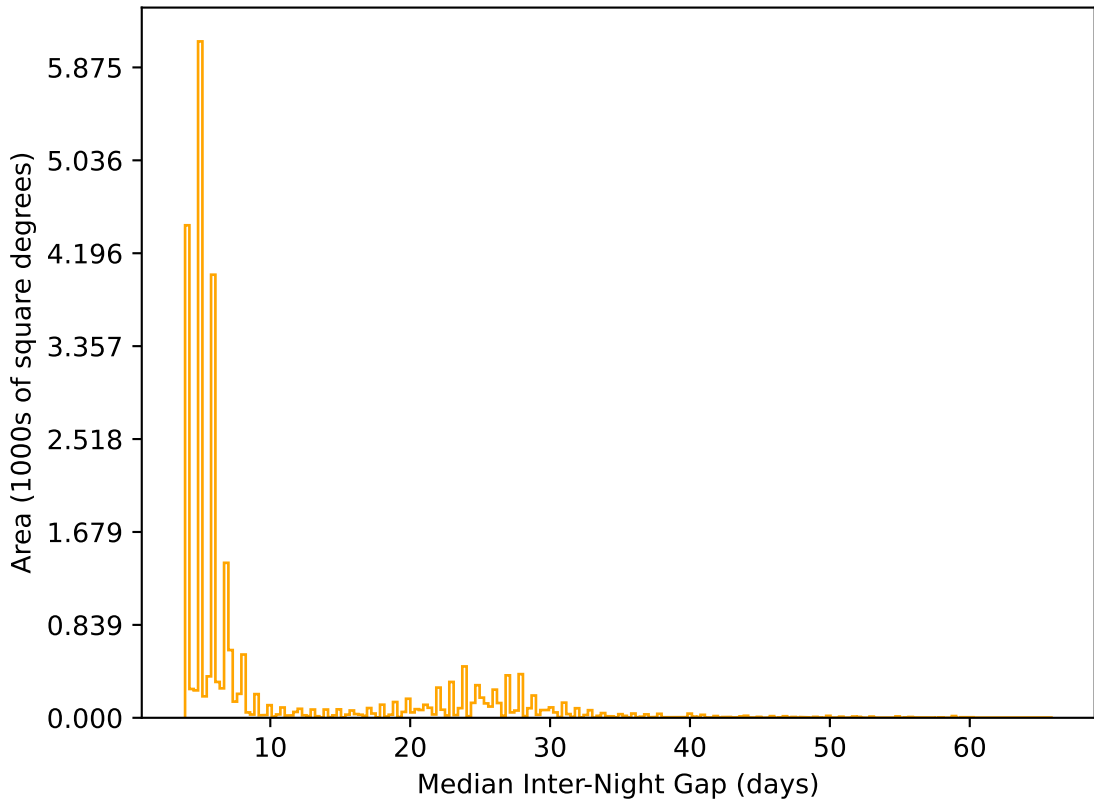
weather_cloudso6v3.4_10yrs All sky r band: Median Inter-Night Gap
