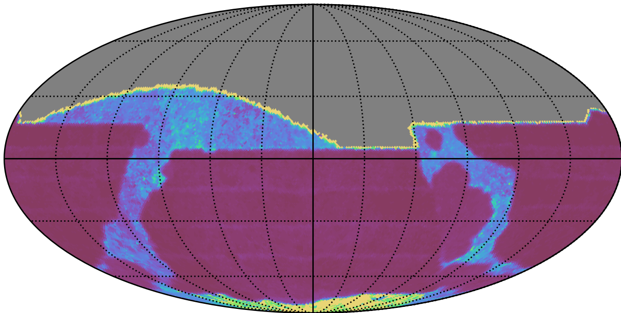
weather_cloudso6v3.4_10yrs All sky i band: Median Inter-Night Gap
