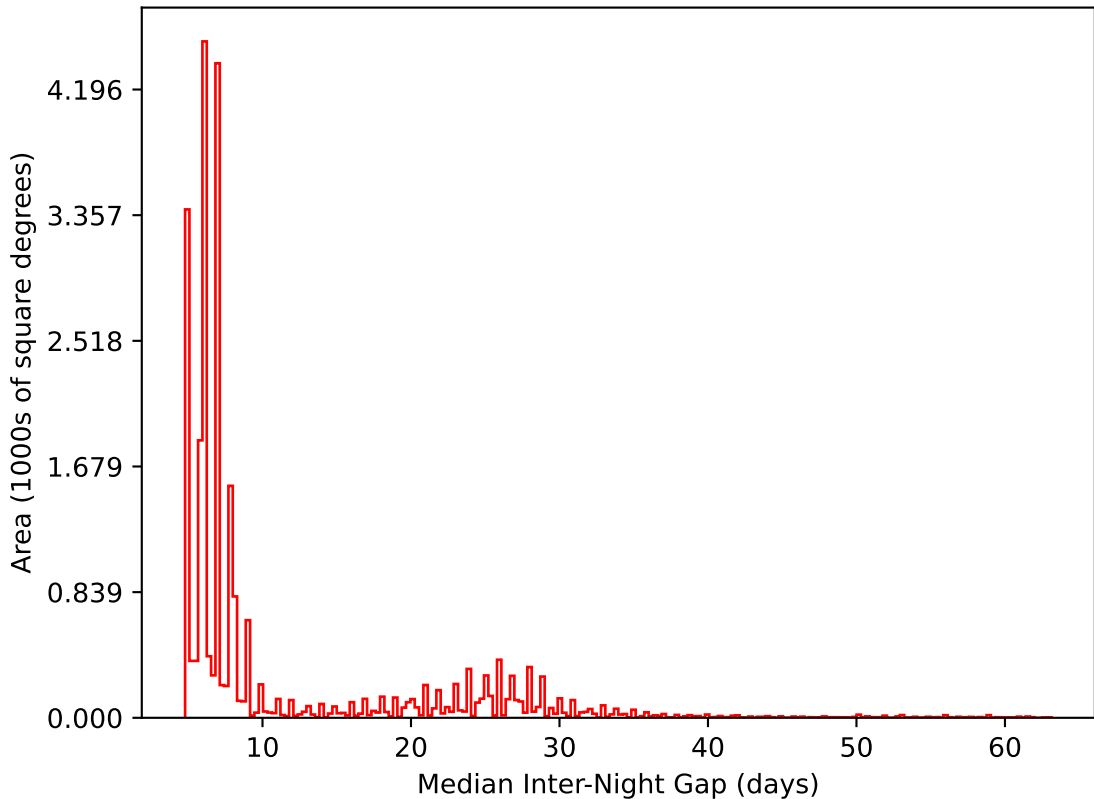
weather_cloudso6v3.4_10yrs All sky i band: Median Inter-Night Gap
