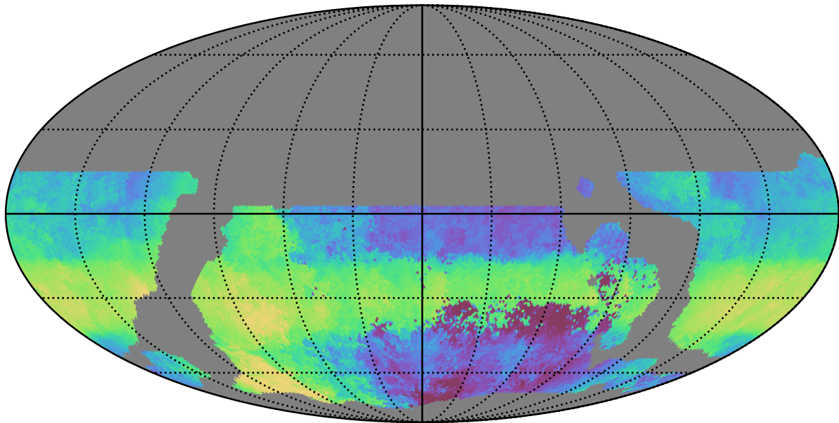
weather_cloudso6v3.4_10yrs WFD u band: Median HA
