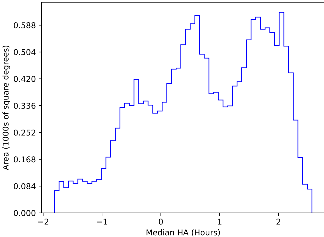
weather_cloudso6v3.4_10yrs WFD u band: Median HA
