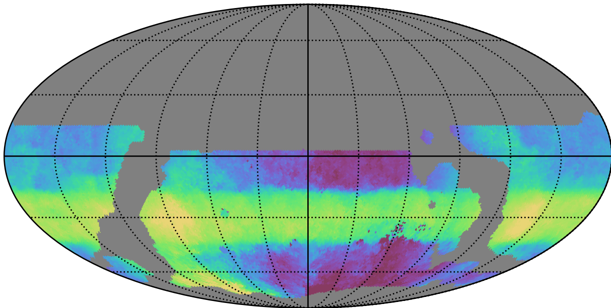
weather_cloudso6v3.4_10yrs WFD r band: Median HA
