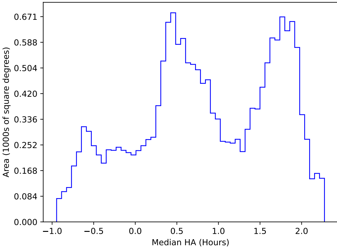
weather_cloudso6v3.4_10yrs WFD r band: Median HA
