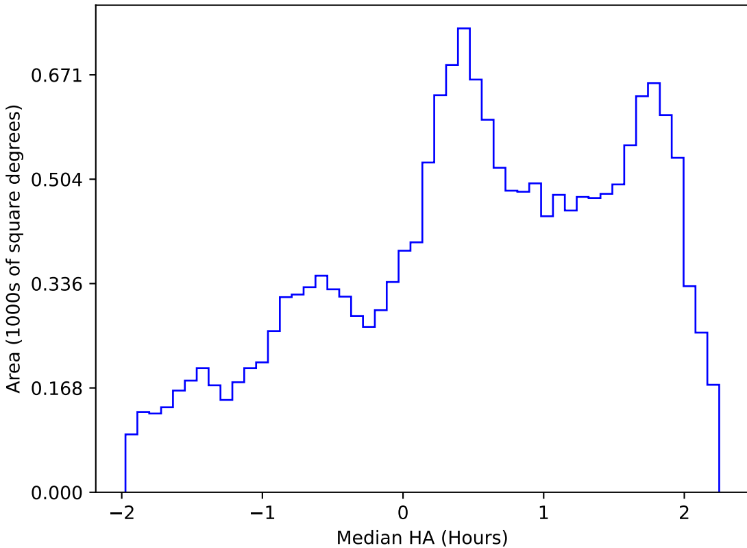
weather_cloudso6v3.4_10yrs WFD g band: Median HA
