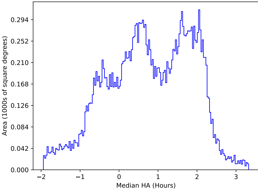
weather_cloudso6v3.4_10yrs All sky u band: Median HA
