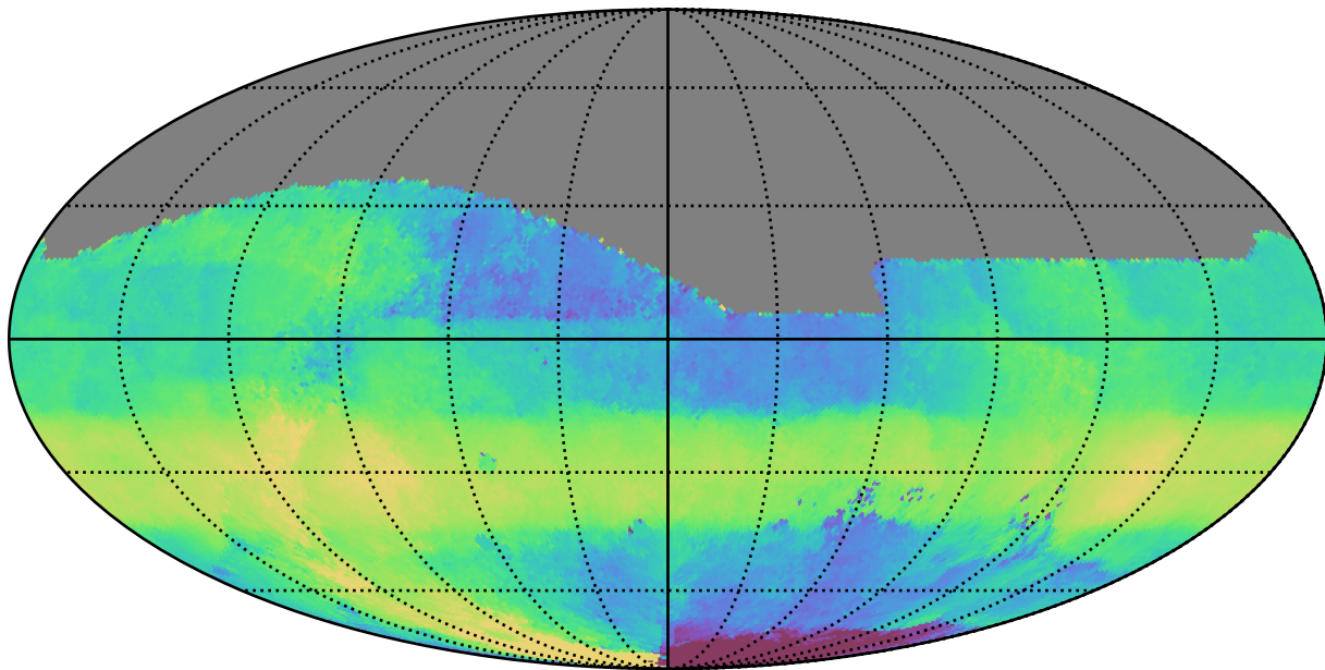
weather_cloudso6v3.4_10yrs All sky r band: Median HA
