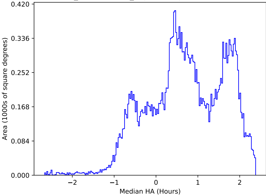
weather_cloudso6v3.4_10yrs All sky r band: Median HA
