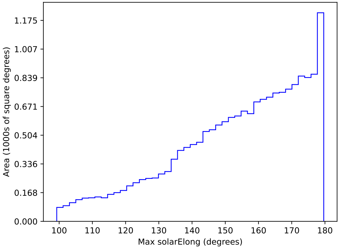
weather_cloudso6v3.4_10yrs WFD all bands: Max solarElong
