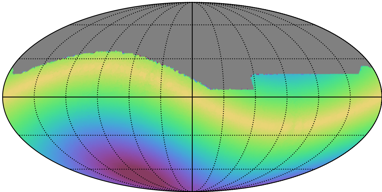
weather_cloudso6v3.4_10yrs All sky all bands: Max solarElong
