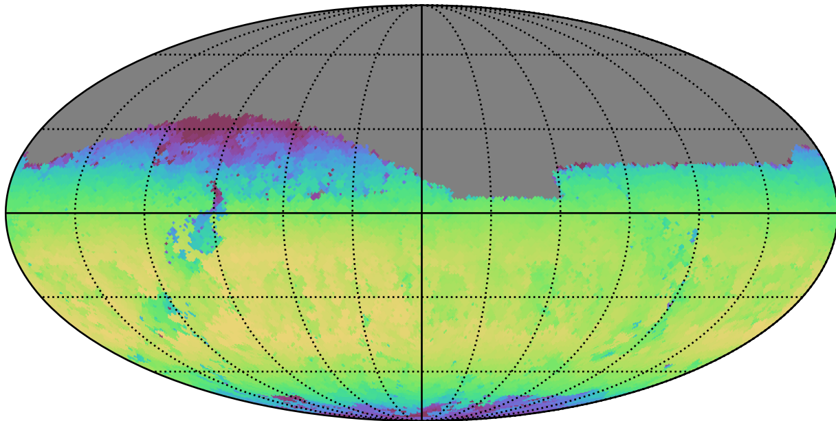
weather_cloudso6v3.4_10yrs Yr 1 z band: Max skyBrightness
