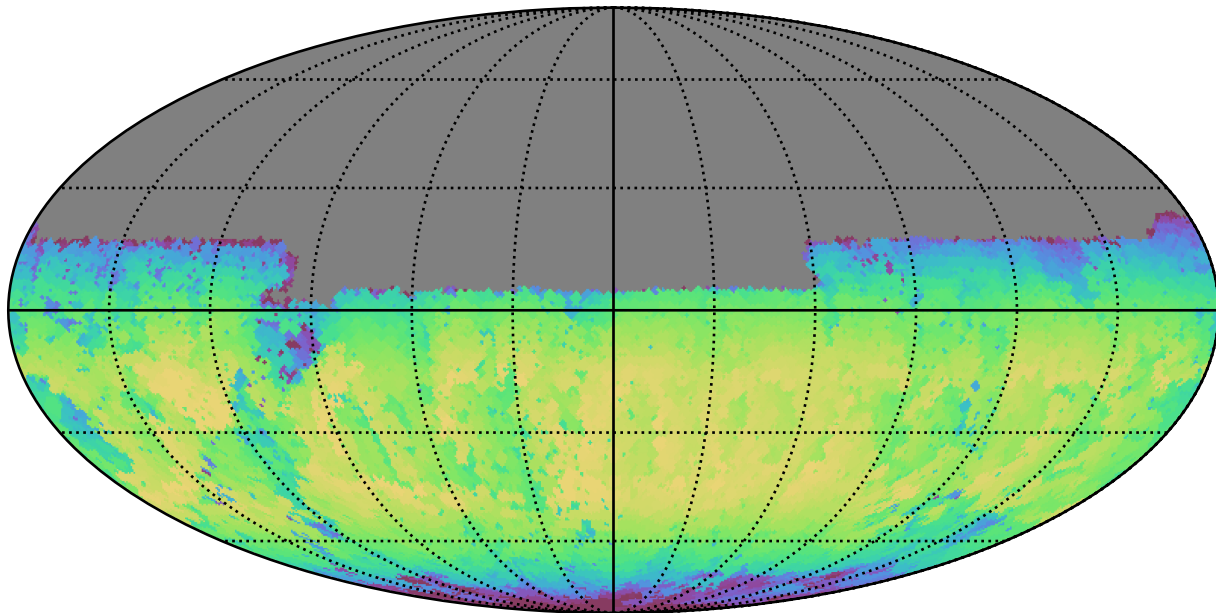
weather_cloudso6v3.4_10yrs Yr 1 y band: Max skyBrightness
