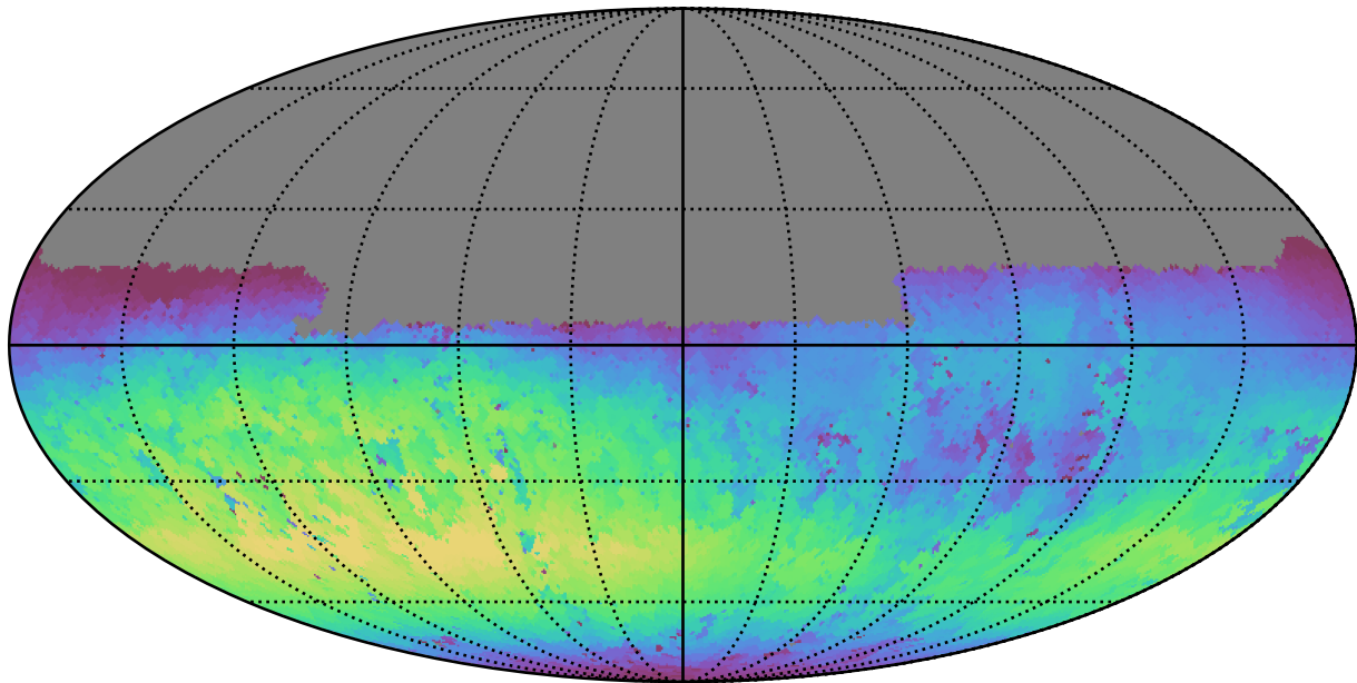
weather_cloudso6v3.4_10yrs Yr 1 u band: Max skyBrightness
