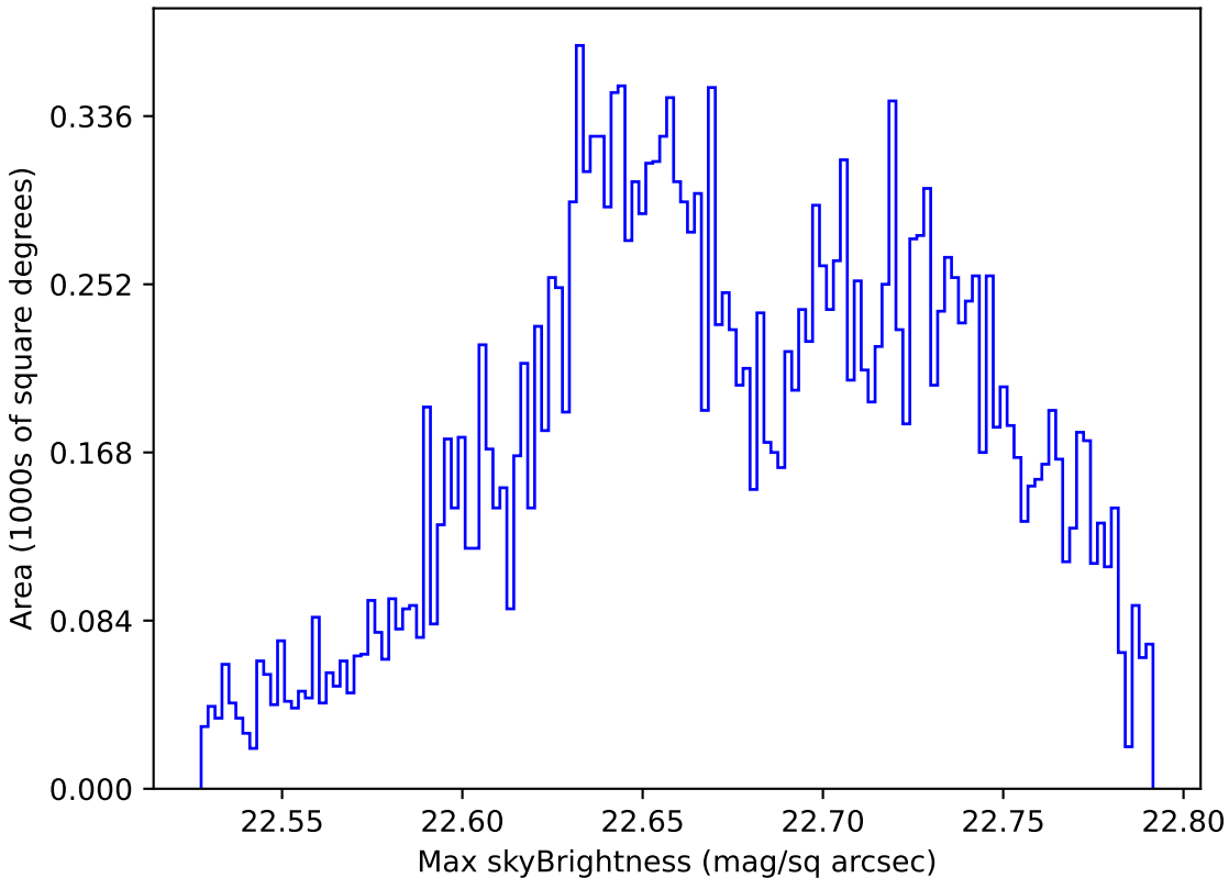
weather_cloudso6v3.4_10yrs Yr 1 u band: Max skyBrightness
