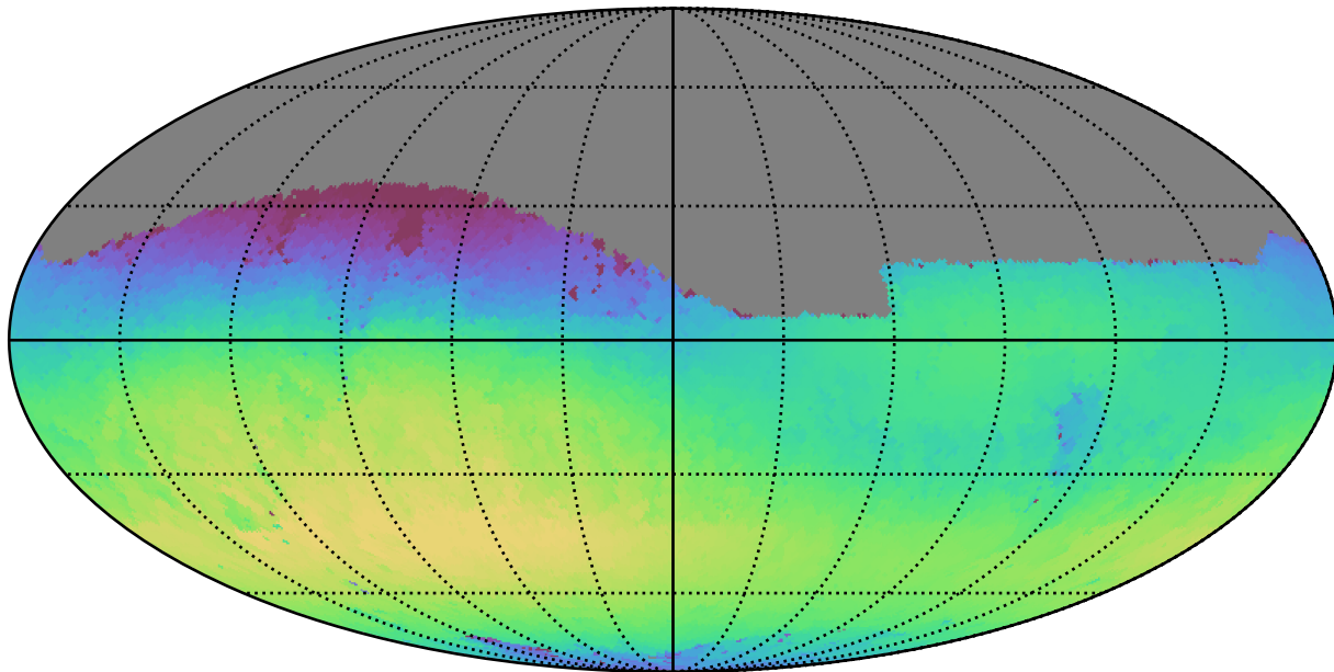
weather_cloudso6v3.4_10yrs Yr 1 r band: Max skyBrightness
