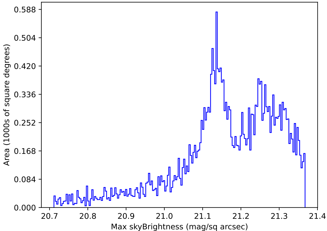
weather_cloudso6v3.4_10yrs Yr 1 r band: Max skyBrightness
