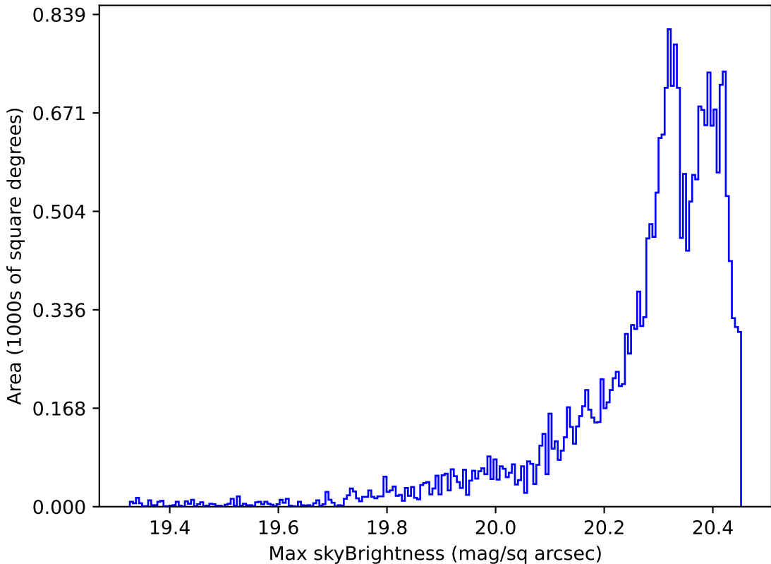
weather_cloudso6v3.4_10yrs Yr 1 i band: Max skyBrightness
