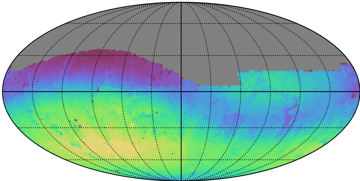
weather_cloudso6v3.4_10yrs Yr 1 g band: Max skyBrightness
