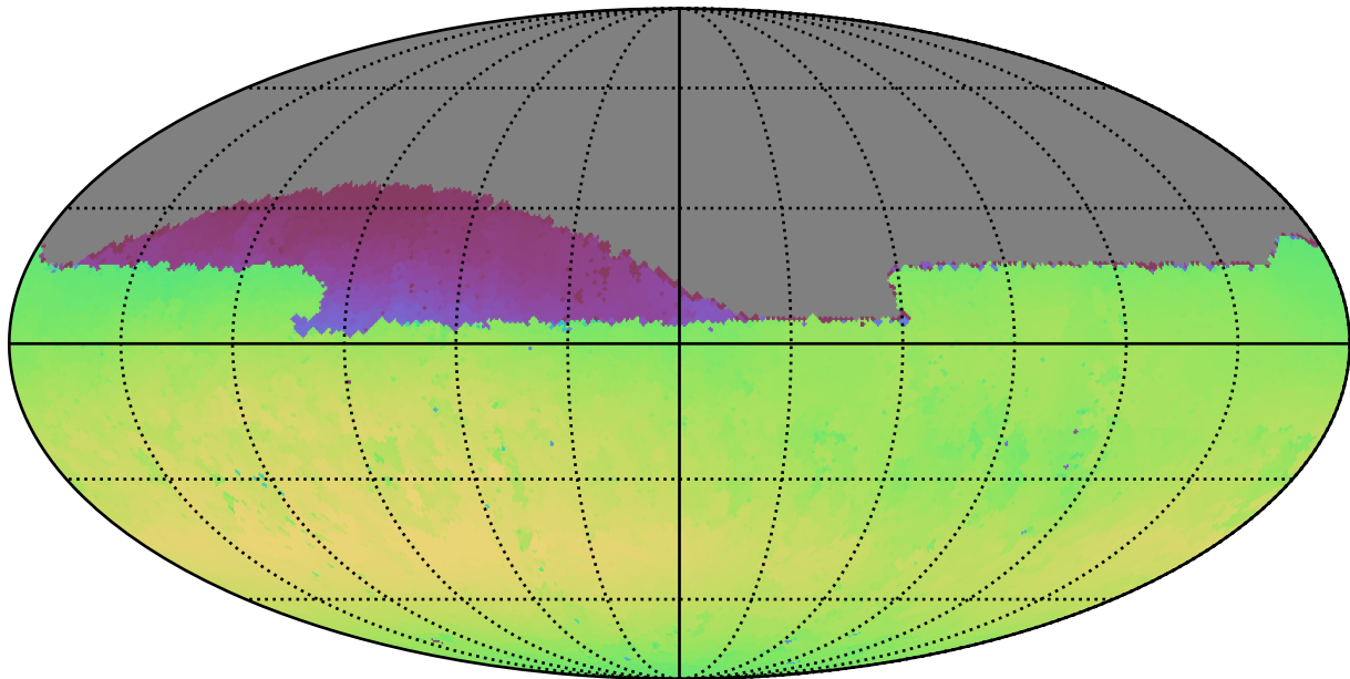
weather_cloudso6v3.4_10yrs Yr1 all bands: Max skyBrightness
