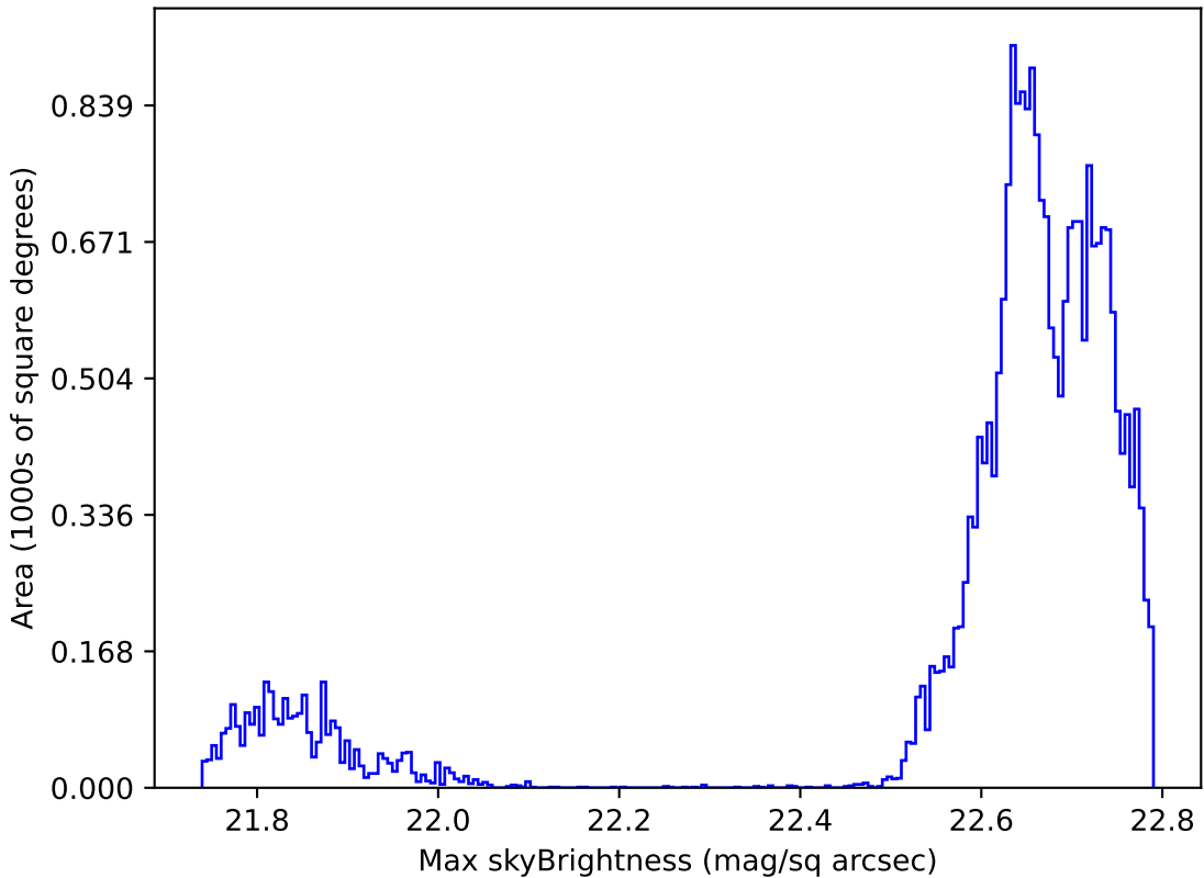
weather_cloudso6v3.4_10yrs Yr 1 all bands: Max skyBrightness
