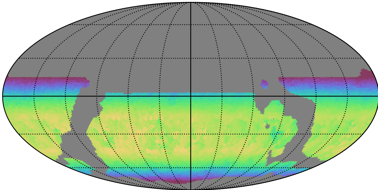
weather_cloudso6v3.4_10yrs WFD y band: Max skyBrightness
