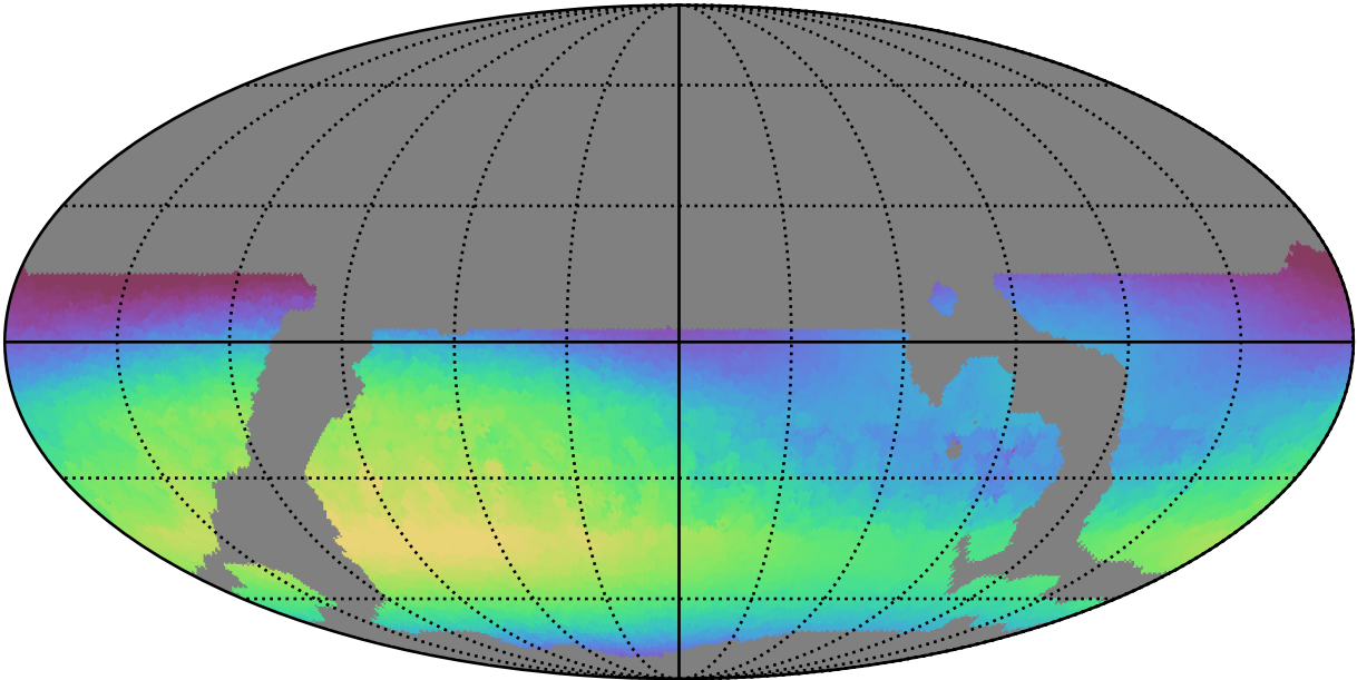
weather_cloudso6v3.4_10yrs WFD u band: Max skyBrightness
