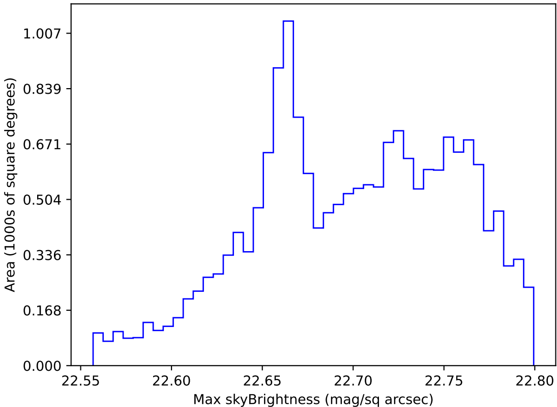
weather_cloudso6v3.4_10yrs WFD u band: Max skyBrightness
