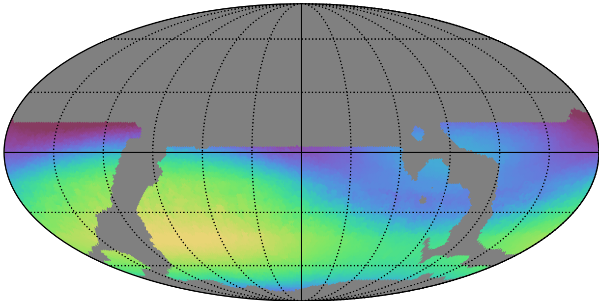
weather_cloudso6v3.4_10yrs WFD r band: Max skyBrightness
