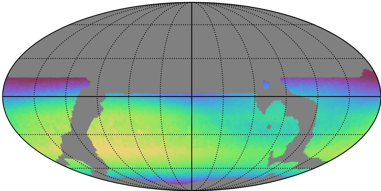
weather_cloudso6v3.4_10yrs WFD i band: Max skyBrightness
