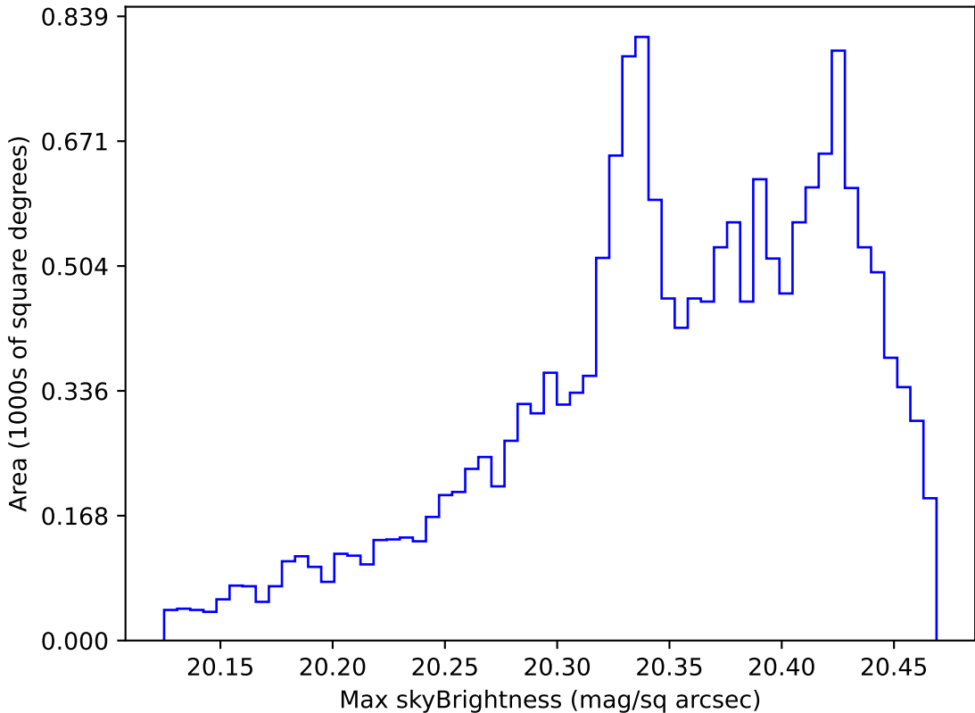
weather_cloudso6v3.4_10yrs WFD i band: Max skyBrightness
