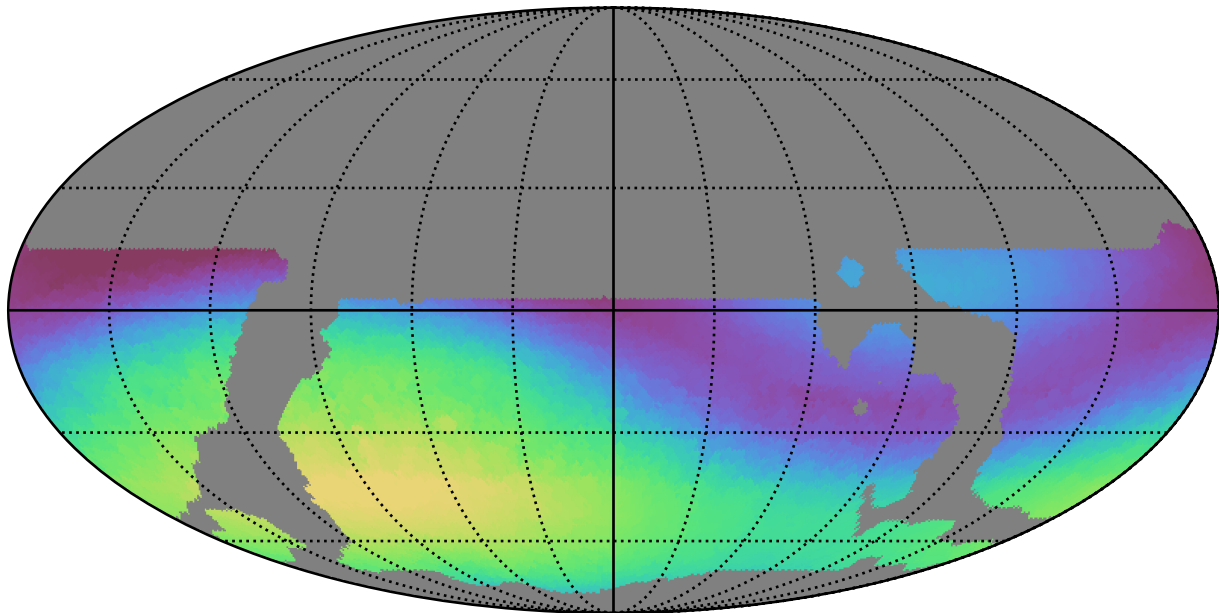
weather_cloudso6v3.4_10yrs WFD g band: Max skyBrightness
