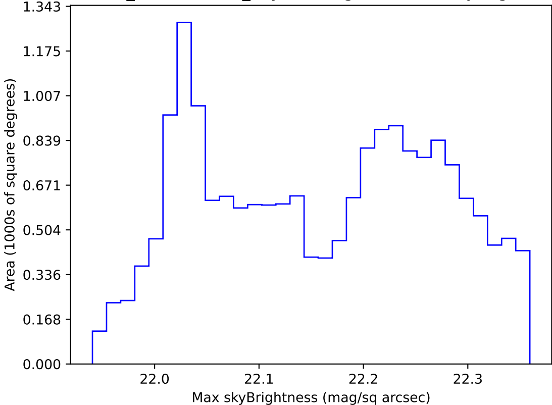
weather_cloudso6v3.4_10yrs WFD g band: Max skyBrightness
