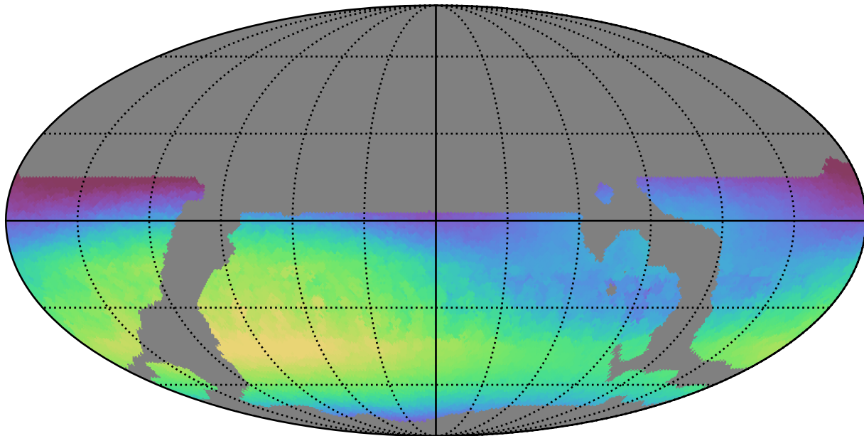
weather_cloudso6v3.4_10yrs WFD all bands: Max skyBrightness
