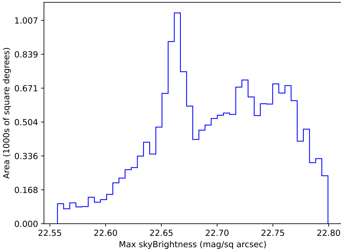
weather_cloudso6v3.4_10yrs WFD all bands: Max skyBrightness
