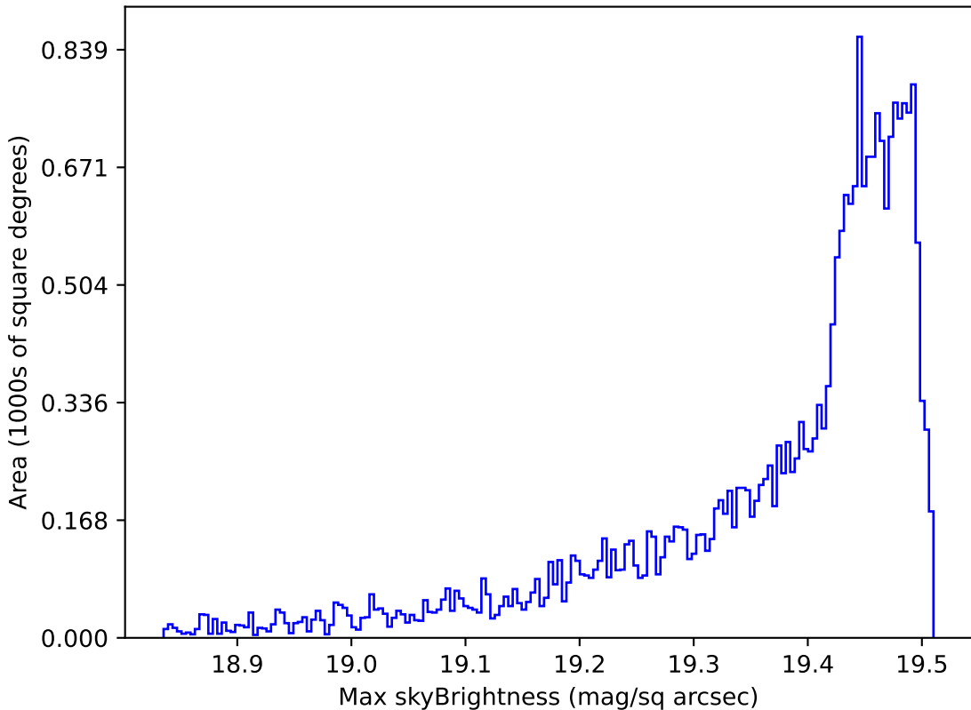
weather_cloudso6v3.4_10yrs All sky z band: Max skyBrightness
