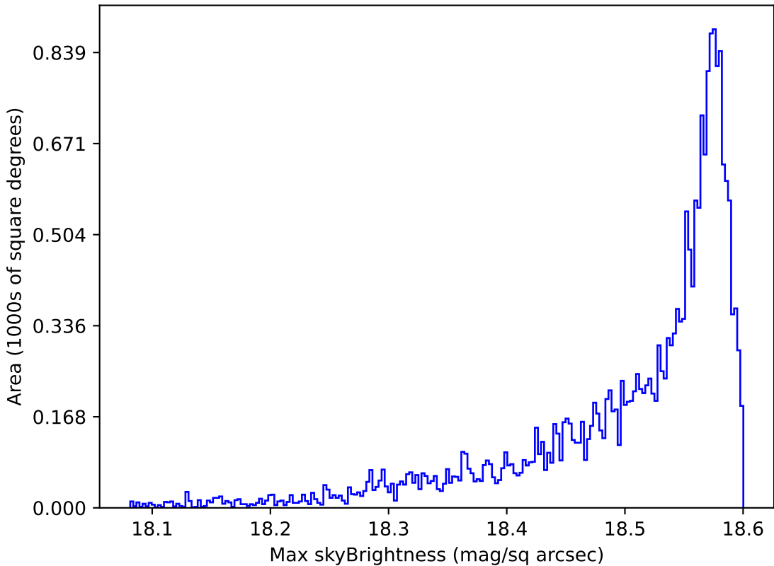
weather_cloudso6v3.4_10yrs All sky y band: Max skyBrightness
