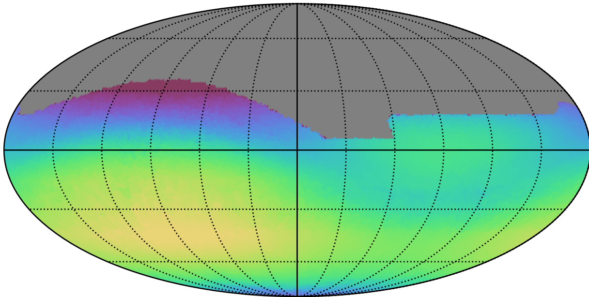
weather_cloudso6v3.4_10yrs All sky r band: Max skyBrightness
