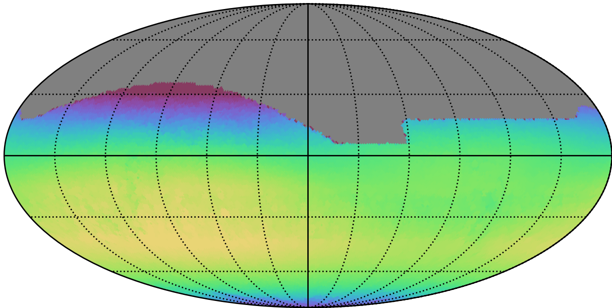
weather_cloudso6v3.4_10yrs All sky i band: Max skyBrightness
