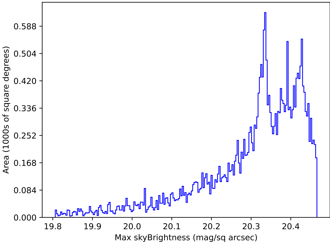
weather_cloudso6v3.4_10yrs All sky i band: Max skyBrightness
