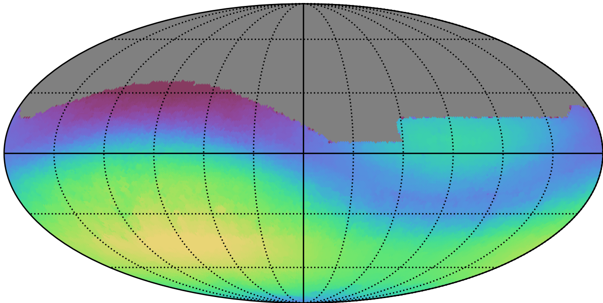
weather_cloudso6v3.4_10yrs All sky g band: Max skyBrightness
