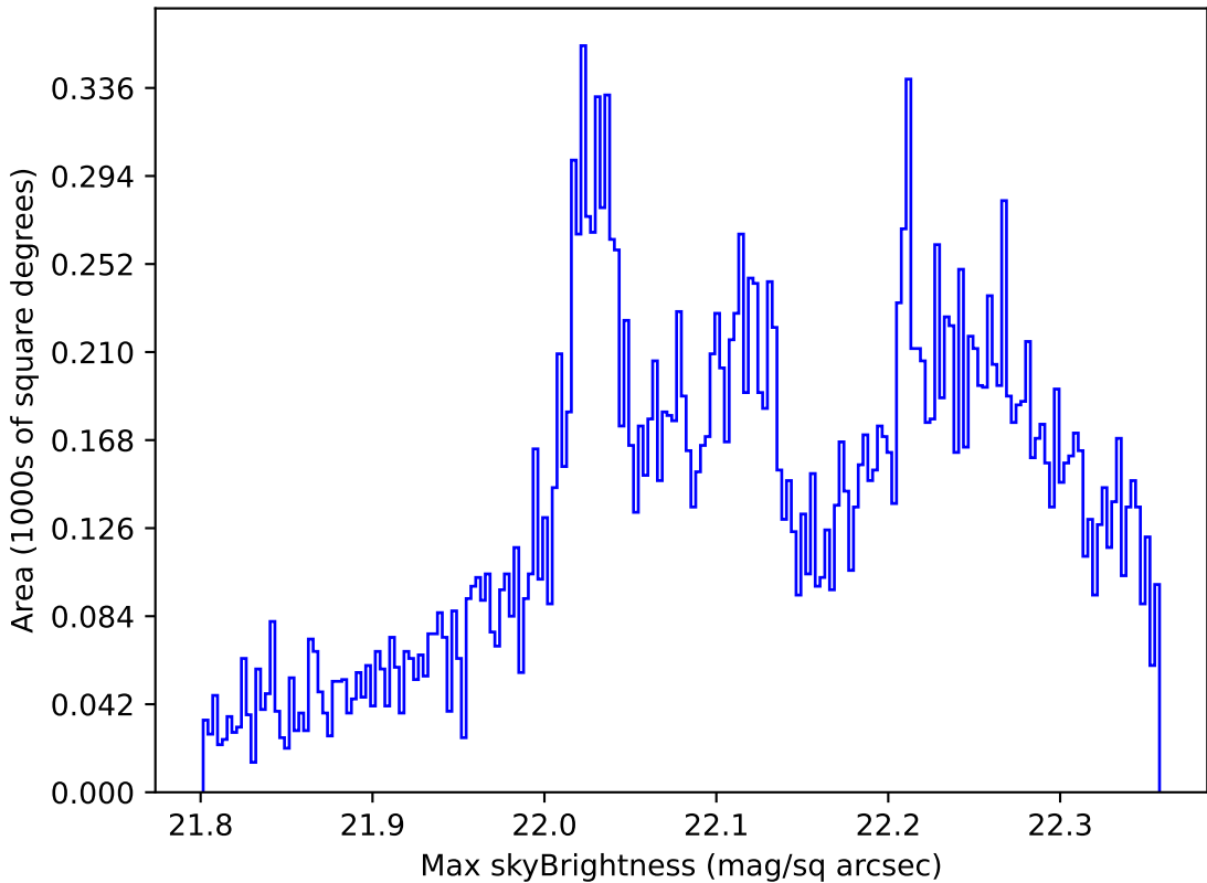
weather_cloudso6v3.4_10yrs All sky g band: Max skyBrightness
