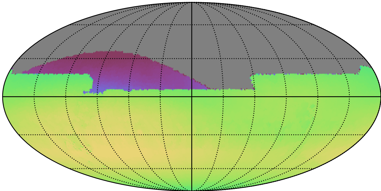
weather_cloudso6v3.4_10yrs All sky all bands: Max skyBrightness
