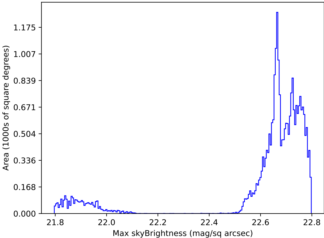
weather_cloudso6v3.4_10yrs All sky all bands: Max skyBrightness
