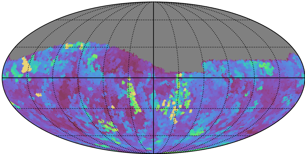
weather_cloudso6v3.4_10yrs Yr 1 z band: Max seeingGeom
